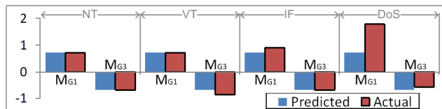
Figure 7. Impact of Feature “Per-Request Authentication” on Metrics “Quote Response Time” and “Quote Quality”.
