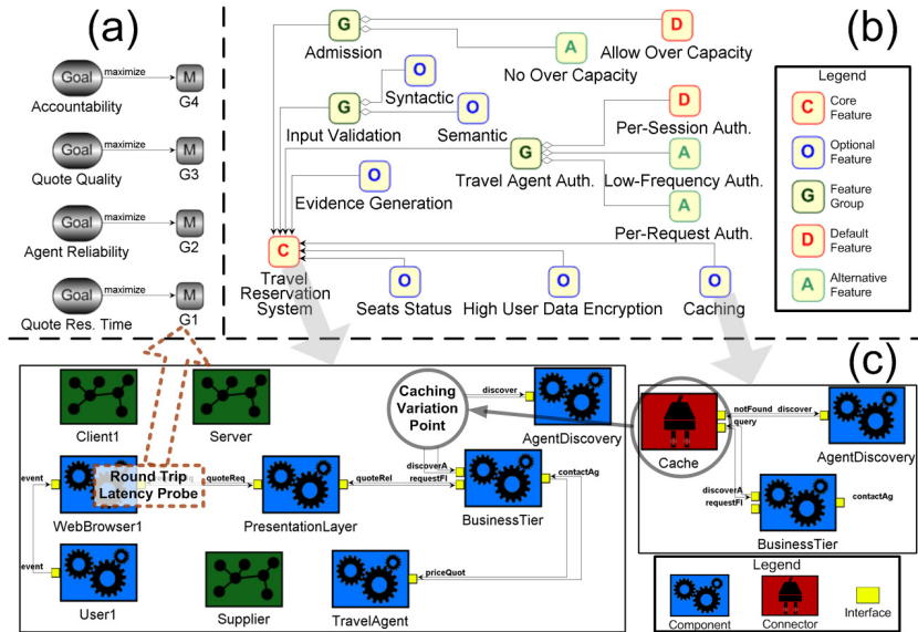
Figure 5. Subset of TRS in our prototype implementation of FUSION: (a) goals and metrics, (b) feature model, (c) implementations of Core and Caching features.
